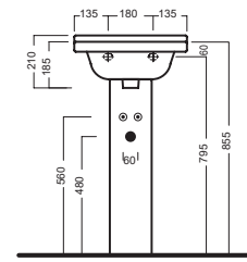
colonna / pedestal
